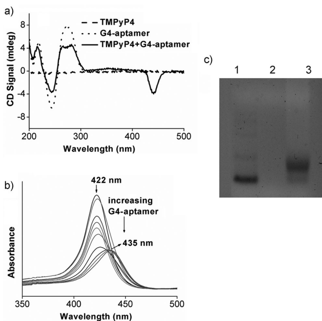
Figure 1. a) CD spectra of TMPyP4 (dashed line), the G4C8 aptamer (dotted line), and the TMPyP4-G4C8 aptamer (solid line). b) UV/Vis absorption titration spectra of TMPyP4 with the G4C8 aptamer. c) Agarose gel electrophoresis tests of the G4C8 aptamer (lane 1), TMPyP4 (lane 2), and the TMPyP4-G4C8 aptamer (lane 3).
