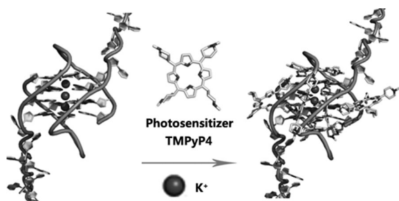
Scheme 2. Interaction between the G4C8 aptamer and TMPyP4.
